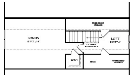
OPT. BONUS SECOND FLOOR PLAN
