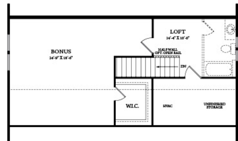
OPT. BONUS SECOND FLOOR PLAN
