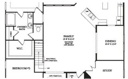
OPT. BONUS FIRST FLOOR PLAN
