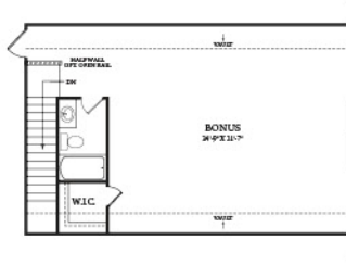
OPT. BONUS & BATH SECOND FLOOR PLAN
