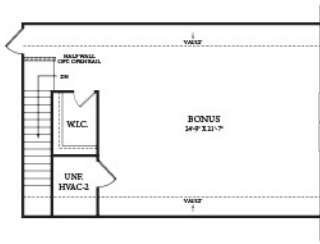
OPT. BONUS SECOND FLOOR PLAN
