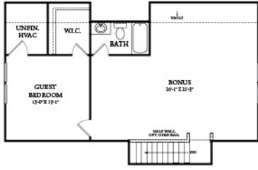
OPT. BONUS, BATH & GUEST BEDROOM SECOND FLOOR PLAN
