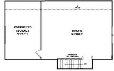
OPT. BONUS & UNFINISHED STORAGE SECOND FLOOR PLAN
